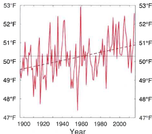
Figure ES-1. The Puget Sound region warmed by +1.3°F from 1895 to 2014. The red line shows average annual temperature for the Puget Sound Lowlands climate division, A the horizontal black line corresponds to the average temperature for 1950–1999 (50.3°F), and the dashed red line is the estimated trend. Data source: Vose et al. 2014. A
