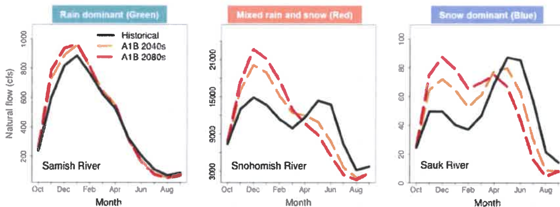
Figure 3-2. Streamflow is projected to increase in winter and decrease in spring and summer for all basin types, with the biggest changes occurring in "mixed rain and snow" watersheds. Results are shown for the Samish River, a warm basin (left); the Sauk River, a cold basin with source waters at high elevations (right) and the Snohomish River, a middle-elevation basin with substantial area near the current snowline (middle). Projections are described in the caption for Figure 3-1. Data source: Hamlet et al., 2013. 24
