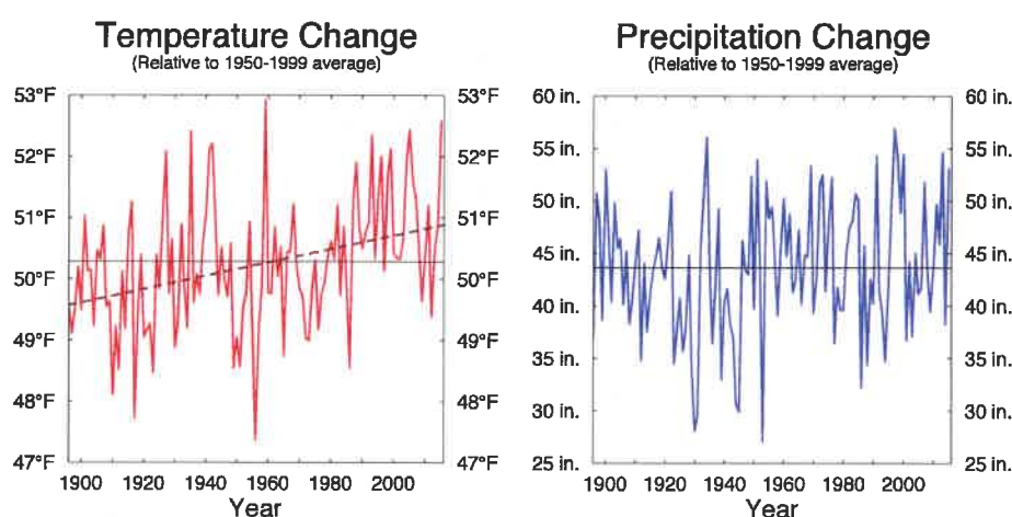
Figure 2-1. Temperature is rising in the Puget Sound lowlands, and there is no long term trend in precipitation. Average annual air temperature (top left, red, in ^{\circ}\text{F} ) and total annual precipitation (top right, blue, in in.) for the Puget Sound Lowlands climate division D (dark blue shading in map), shown relative to the average for 1950-1999 (black horizontal line in both graphs, corresponding to 50.3^{\circ}\text{F} for annual average temperature and 43.6 inches for annual total precipitation). The dashed line in the temperature plot is the fitted trend, indicating a warming of +1.3^{\circ}\text{F} (range: +0.7^{\circ}\text{F} to +1.9^{\circ}\text{F} ) B from 1895 to 2014. The trend for precipitation is not statistically significant, and therefore is not shown. Data source: Vose et al. 2014. D,1
