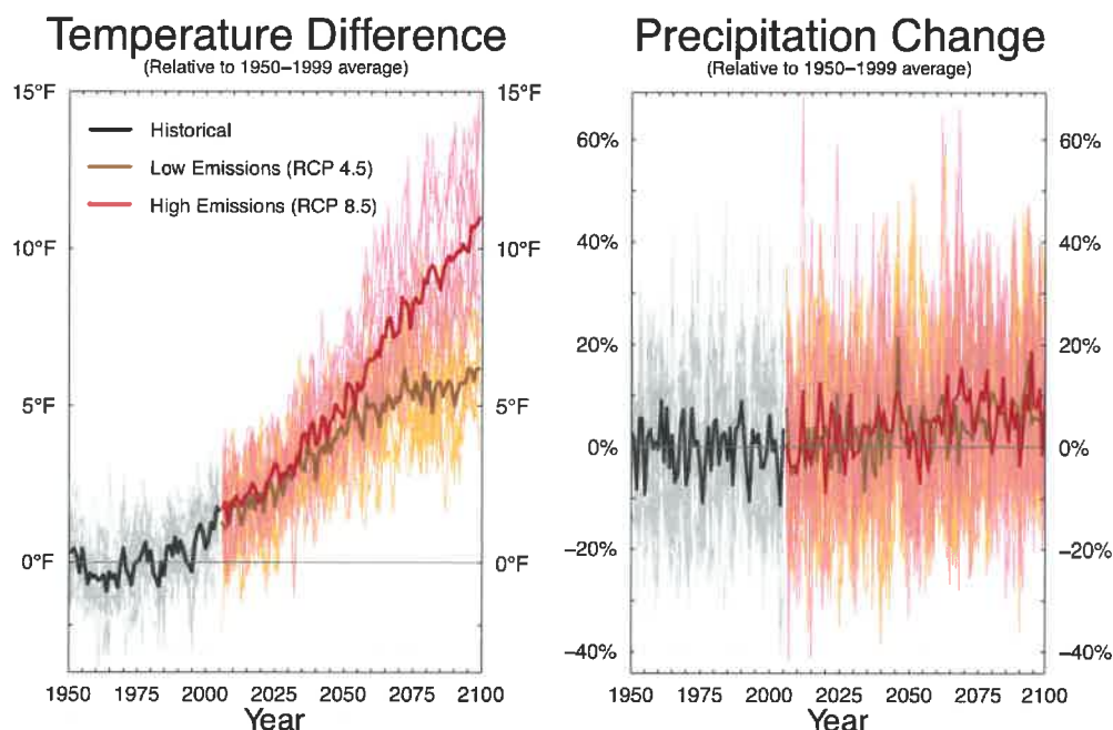
Figure 2-2. All scenarios project warming in the Puget Sound region for the 21 st century; projected changes in annual precipitation are small compared to year-to-year variability. The graphs show average yearly air temperature and precipitation for the Puget Sound region, relative to the average for 1950–1999 (horizontal gray line, corresponding to an annual average temperature of 44°F and an annual total precipitation of 78 inches). The black line shows the average simulated air temperature or precipitation for 1950–2005, based on the individual model results indicated by the thin grey lines. The thick colored lines show the average among model projections for two emissions scenarios (low: RCP 4.5, and high: RCP 8.5 – see Section 1), while the thin colored lines show individual model projections for each scenario. Data source: Downscaled climate projections developed by Abatzoglou and Brown (2011). 26,23,27
