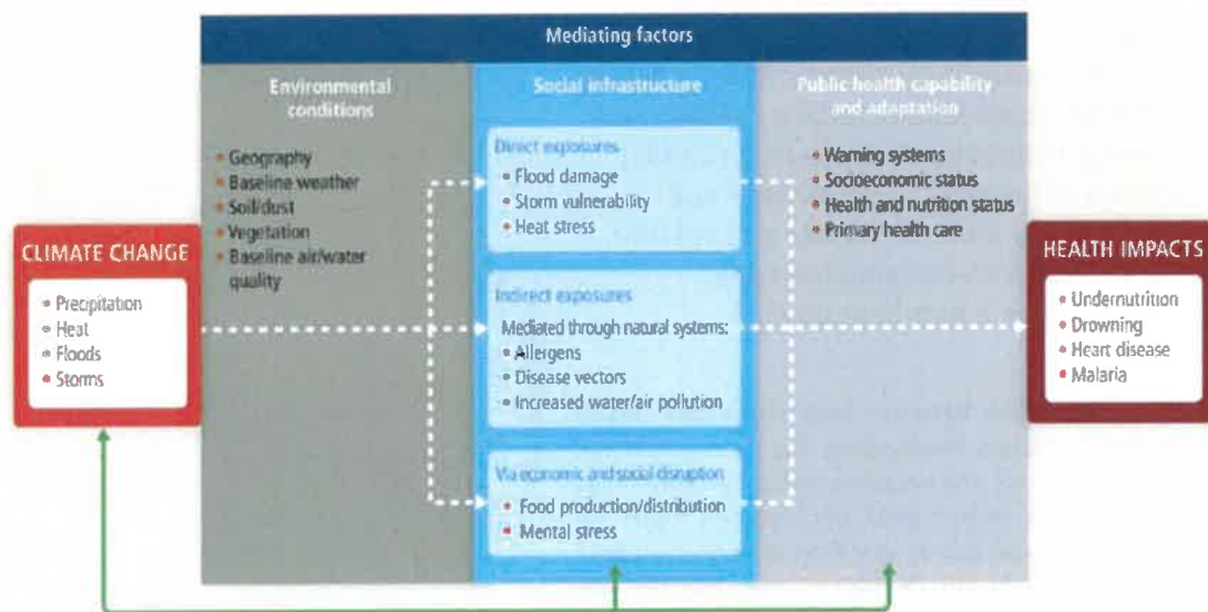
Figure 13-1. Conceptually, there are three primary ways that climate change affects health: directly through climate and weather; indirectly through natural systems that are influenced by climate; and indirectly via effects on economic and social well-being. Health effects occur when climate change influences a region's baseline environmental conditions (green box) creating new or differing exposure pathways (blue box). These effects can be further modified by factors such as the public health system's existing infrastructure and adaptive capacity (gray box). Green arrows show how some of these factors may be affected by one another. Figure Source: IPCC (2013). 8
